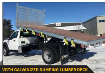
VOTH GALVANIZED DUMPING LUMBER DECK
